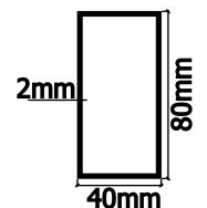
Roof tension tube
