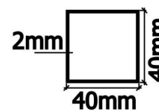
Intermediate purlin
